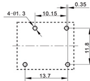
Mounting Dimensions
